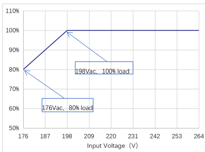
Derating Curve
